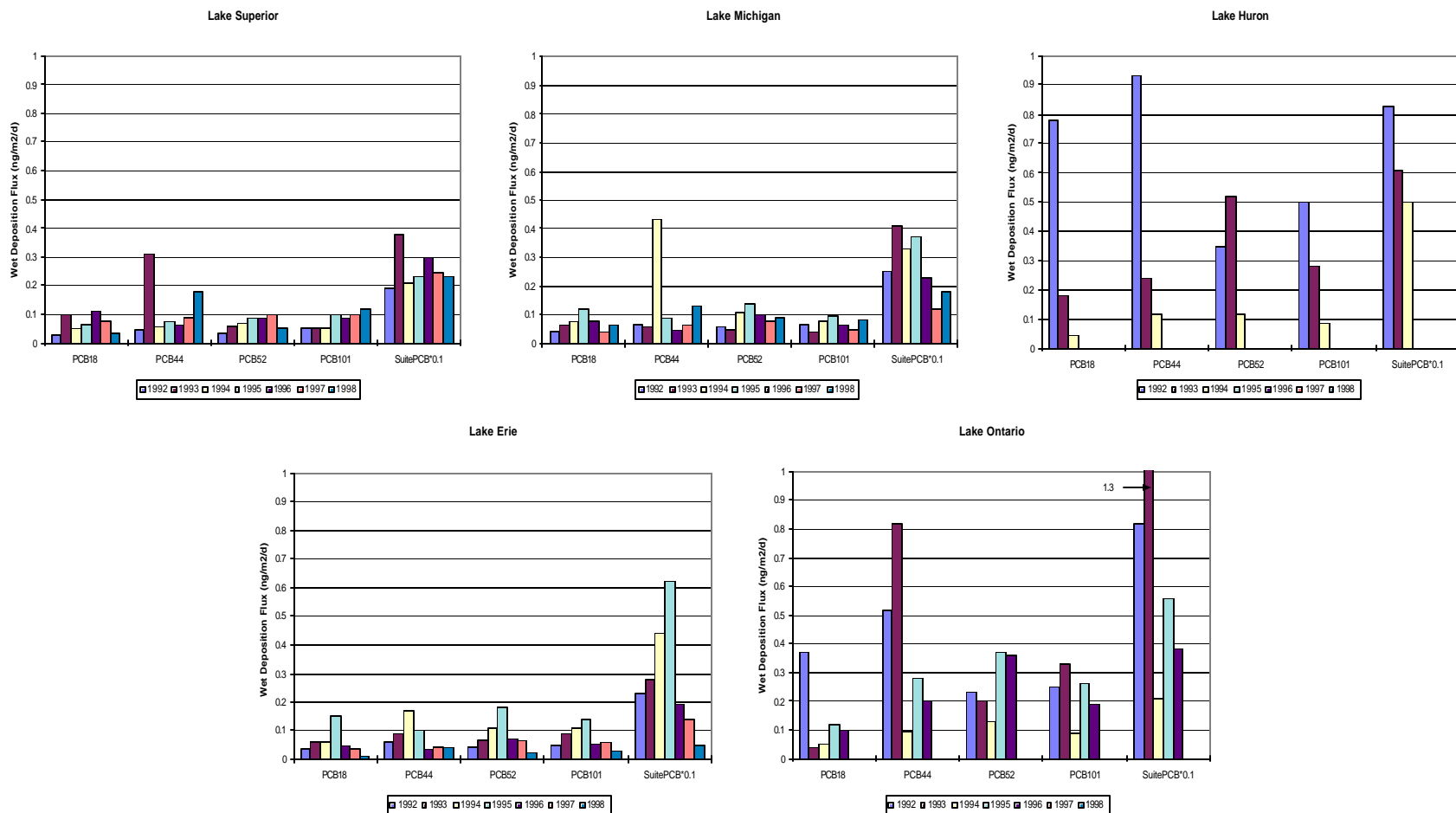
Figure E5. Annual average wet deposition flux (ng/m 2 /day) of PCBs. Note that sum-PCB is multiplied by 0.10.
