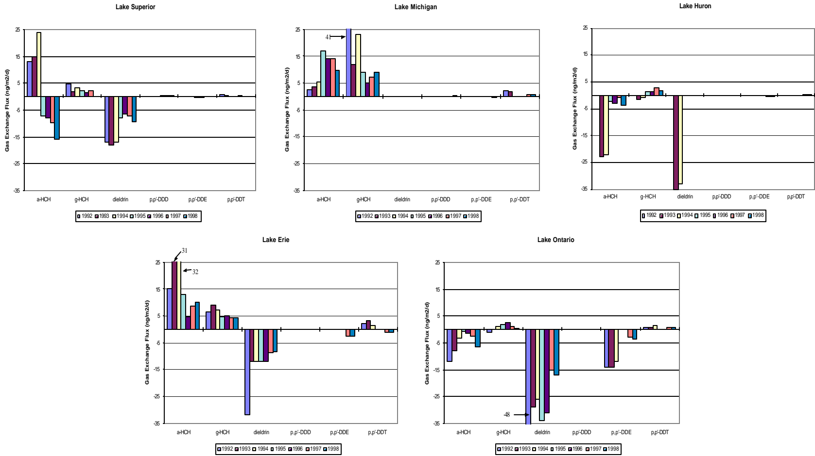
Figure E3. Annual average net gas exchange flux (ng/m 2 /day) of organochlorine pesticides. Positive values denote net gas absorption, negative values denote net volatilization.
