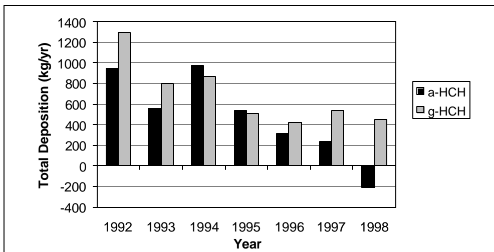
Figure 3. Total flows of a- and g-HCH (kg/yr) over all Great Lakes
