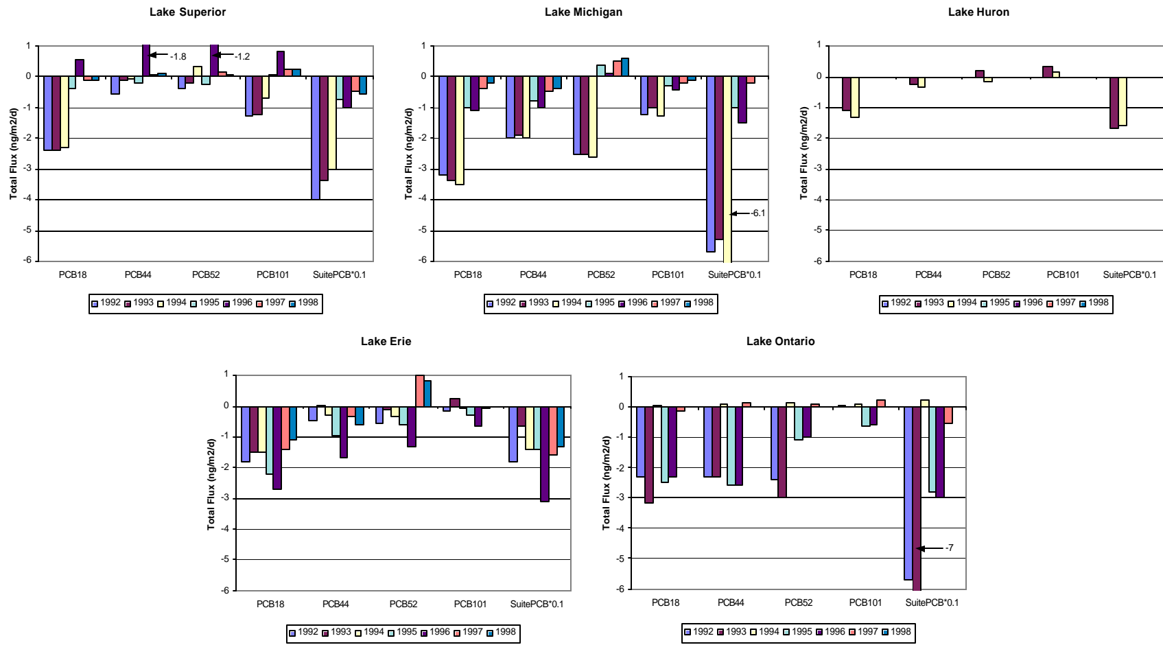
Figure E8. Annual average total flux (ng/m 2 /day) of PCBs. Note that sum-PCB is multiplied by 0.10.
